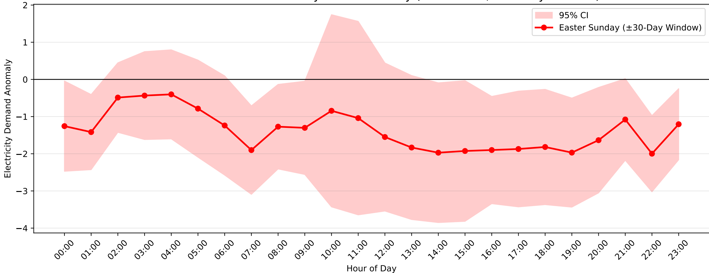
Adamstown Demand Anomaly: Easter Sunday (2004–2017, \pm 30 -Day Window)
